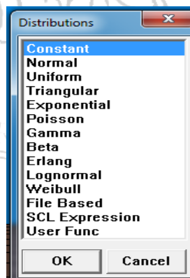
Fig. 1. Statistical distribution.
