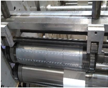
Fig. 6. Die cutting a width of material narrower than the die itself wears out the die.
