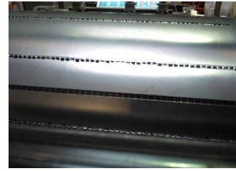
Fig. 13. Destroyed die in the perforation area. It is mounted on the magnetic cylinder
